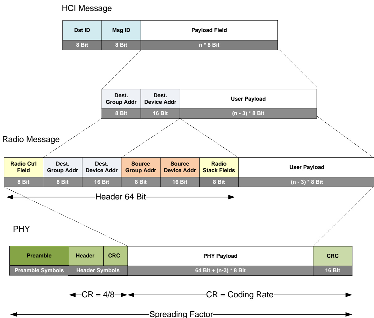
Figure 8-1: iM880B packet structure
